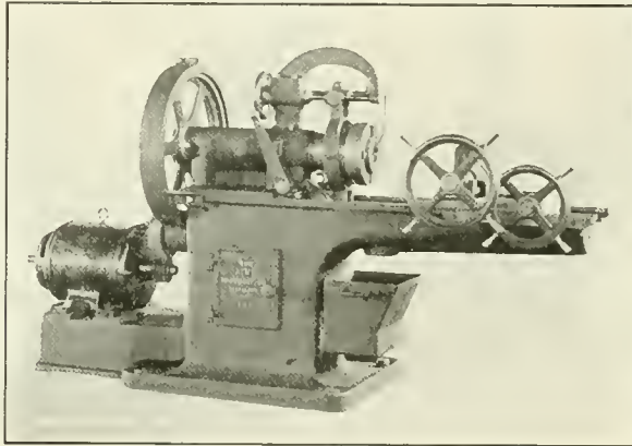
ACME 2-INCH BOLT CUTTER.
